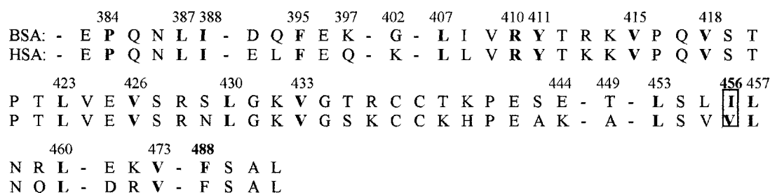
Fig. 1. (A) Structures of lactone and carboxylate forms of 20(S)-CPT and its synthetic stereoisomer 20(R)-CPT. (B) Amino acid sequences of BSA and HSA in the regions of IIA and IIIA principle ligand-binding structural domains. Amino acid residues forming 3D structural ligand-binding domains [17] are in bold-face. Amino acid residues forming 3D structural ligand-binding domains in HSA and replaced by others in BSA are in bold-face and encircled. Deletions in the primary structures correspond to the regions of total homology of the HSA and BSA. Panel B is modified from [16].
