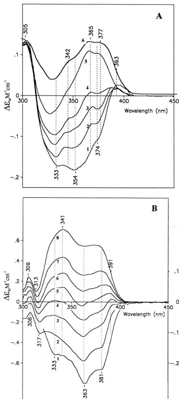
Fig. 2. (A) Hydrolysis kinetics (1–6) of the monomeric form of 20( S )-CPT in PBS, pH 7.4. CD spectra were recorded in 10 min (1); 25 min (2); 40 min (3); 55 min (4); 150 min (5); 230 min (6). (B) Hydrolysis kinetics (2–8) of the monomeric form of 20( S )-CPT in complex with HSA in PBS buffer, pH 7.4. CD spectra were recorded in 10 min (2); 25 min (3); 40 min (4); 55 min (5); 70 min (6); 100 min (7); 230 min (8). Spectrum 1 (panel B) is the CD spectrum of 20( S )-CPT in DMSO solution. Scale for spectrum 1 is presented on the right-hand side. Concentration of 20( S )-CPT in all experiments: 4 \times 10^{-5} M. Concentration of HSA: 4 \times 10^{-5} M.
